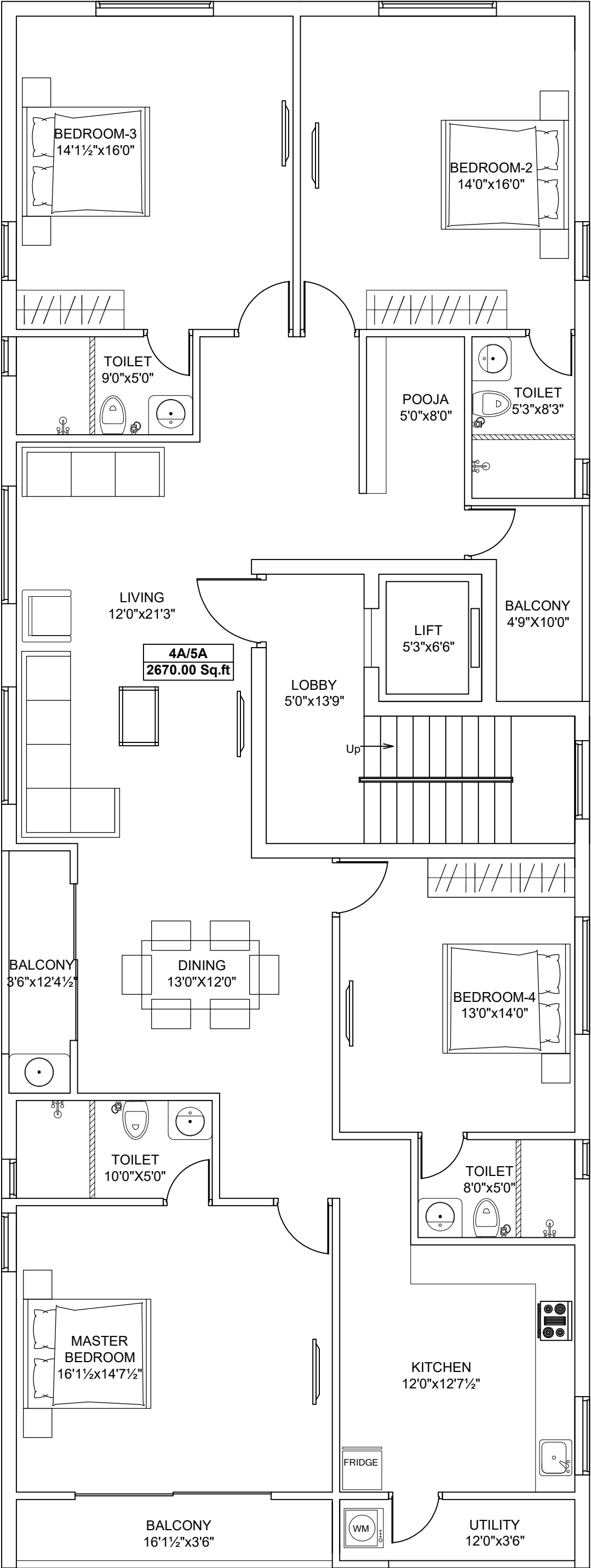
TYPICAL FLOOR PLAN IV,V S BLOCK 4TH MAIN ROAD
